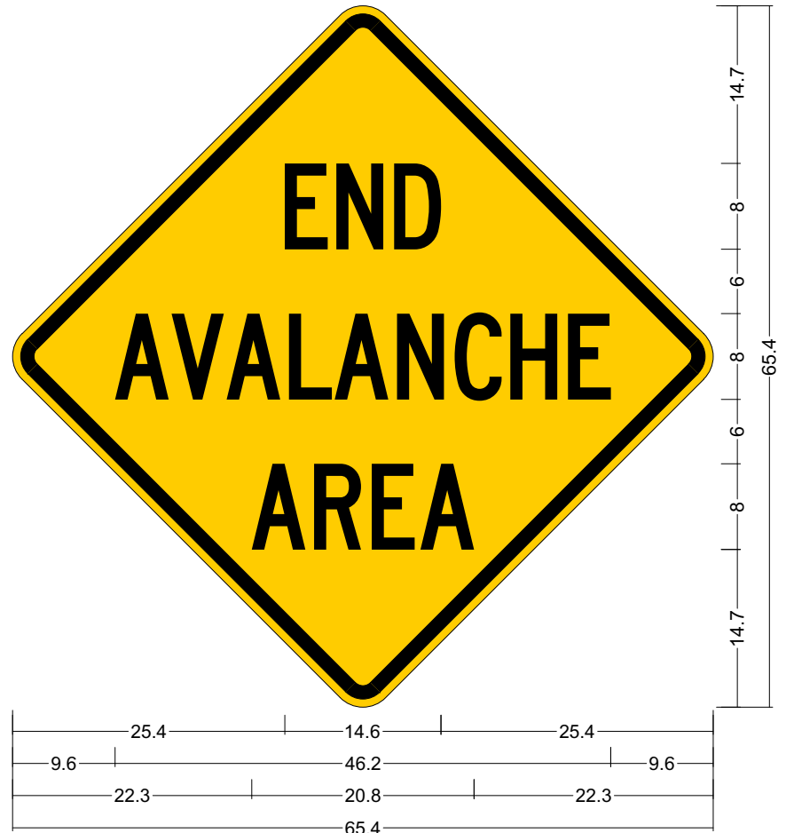
W12-53a End Avalanche Area 48" Across Sides; 48.0" across sides 3.0" Radius, 1.3" Border, 0.8" Indent, Black on Yellow; "END", C 60% spacing; "AVALANCHE", C 60% spacing; "AREA", C 60% spacing;
